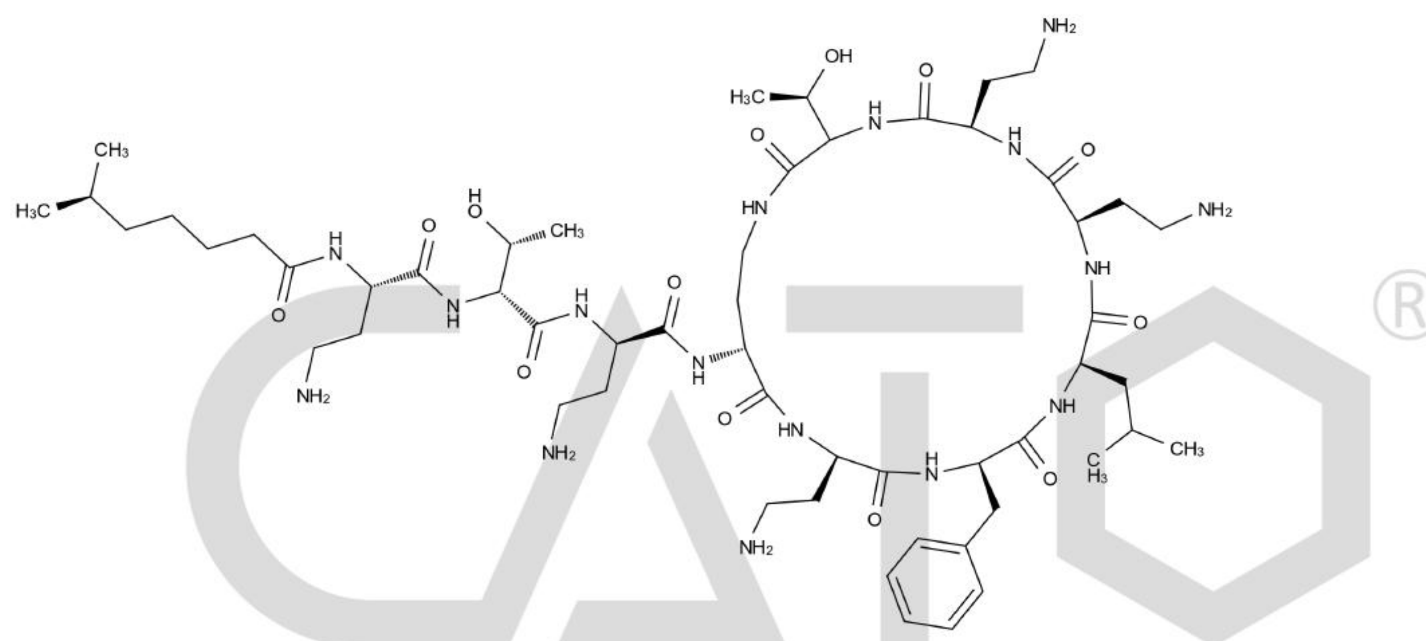
Chemical Structure:
