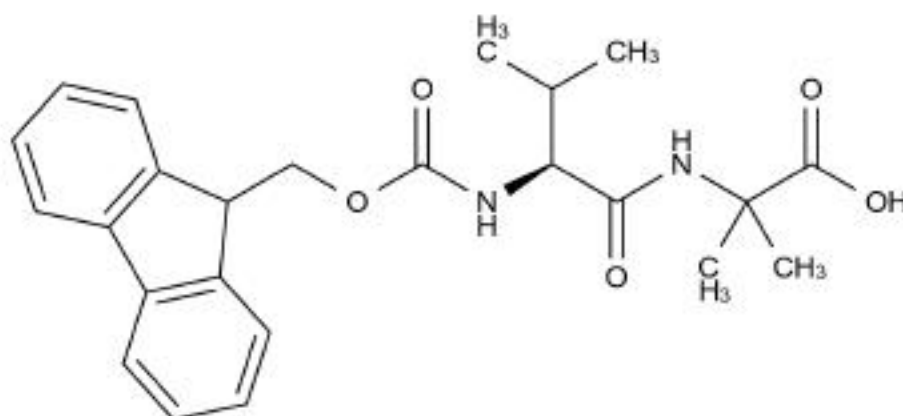
Chemical Structure:
