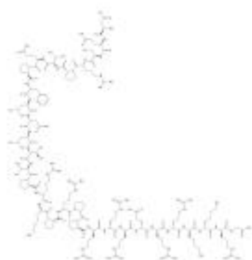
Chemical Structure:
