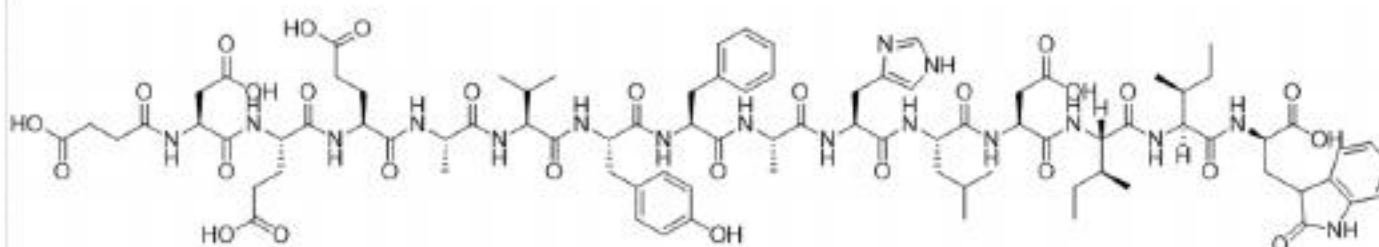
Chemical Structure:
