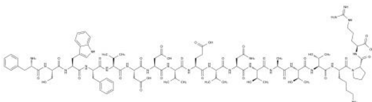
Chemical Structure:
