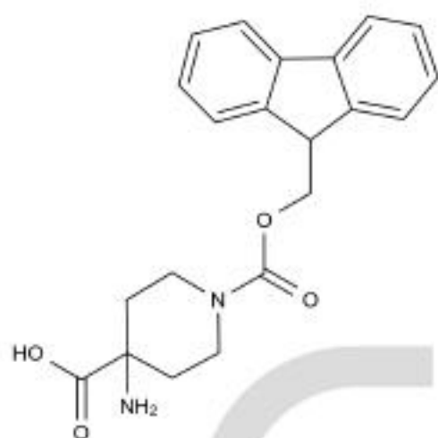
Chemical Structure:
