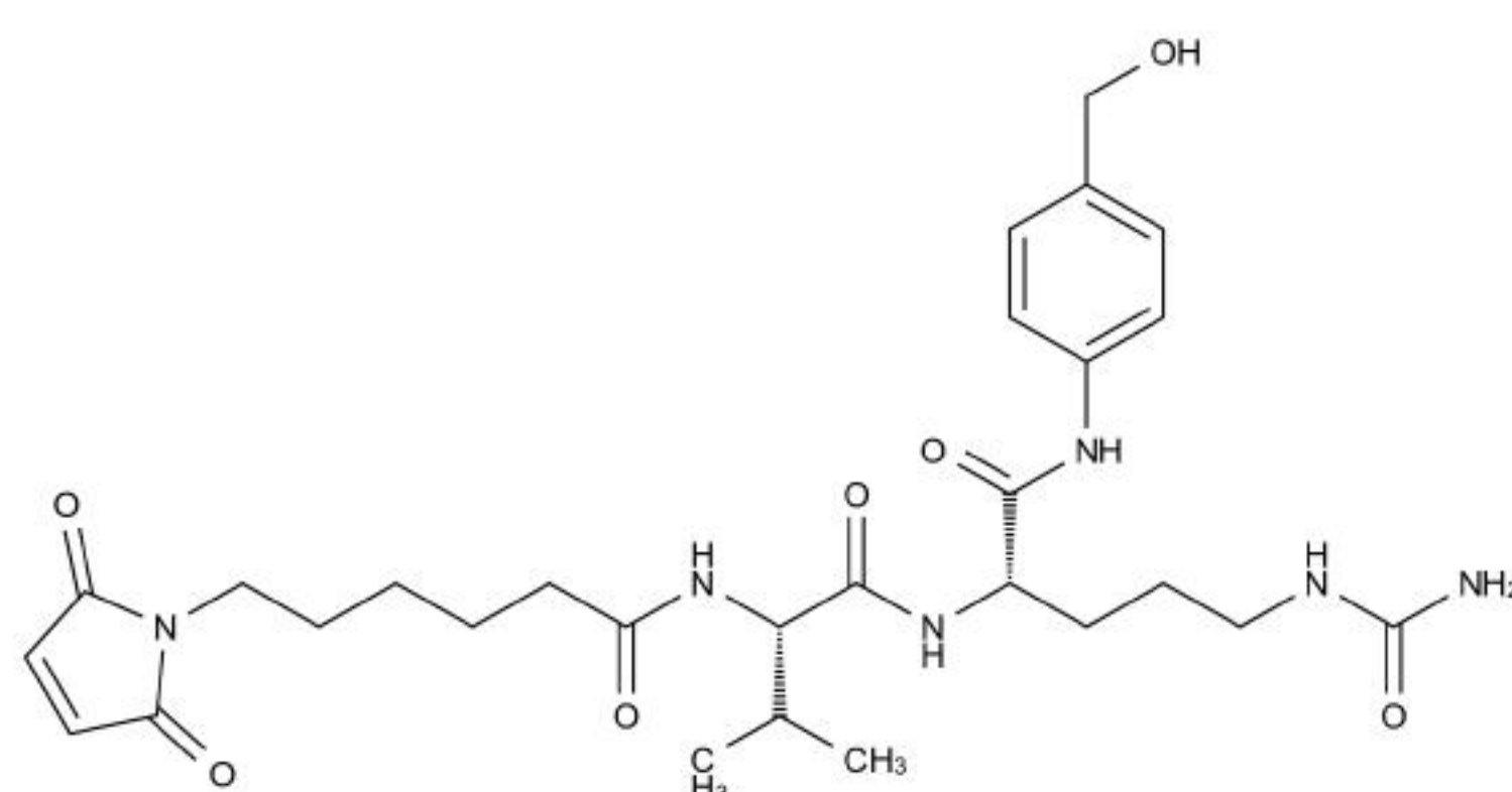
Chemical Structure:
