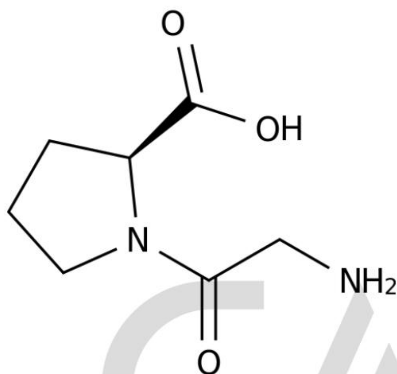
Chemical Structure:
