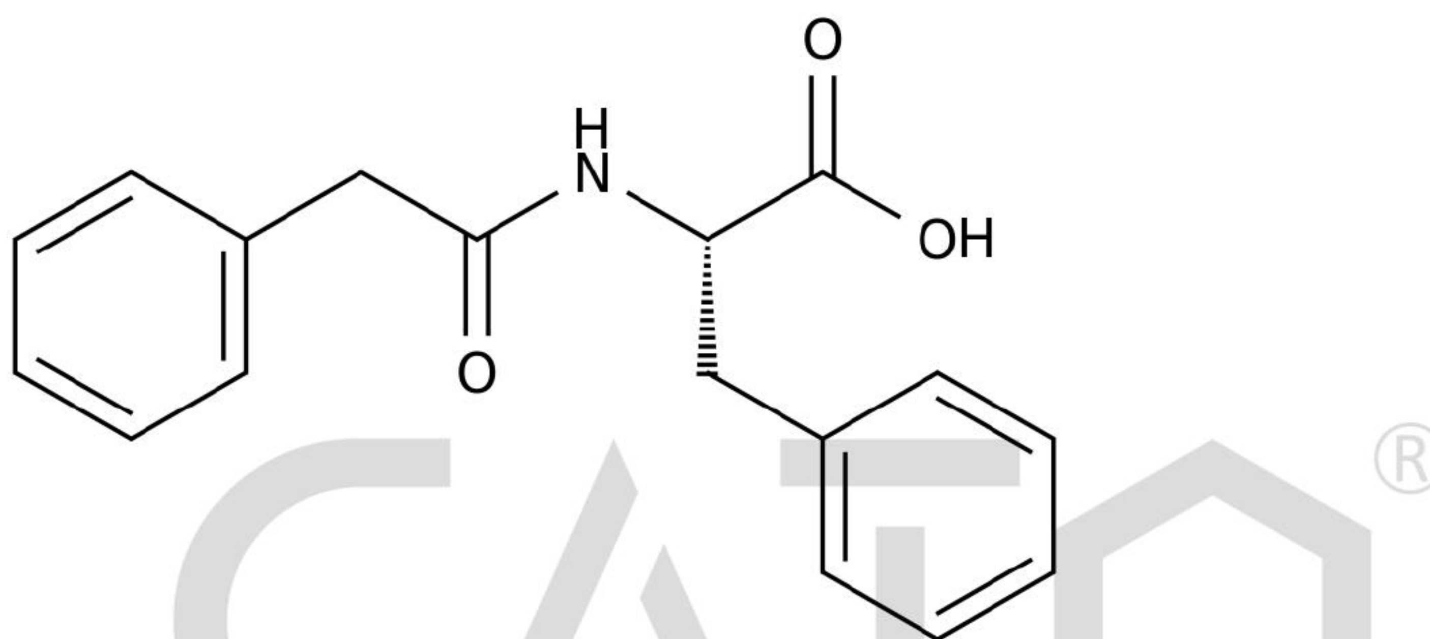
Chemical Structure:
