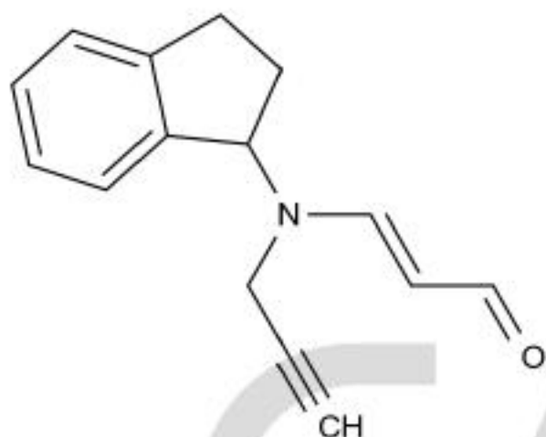
Chemical Structure:
