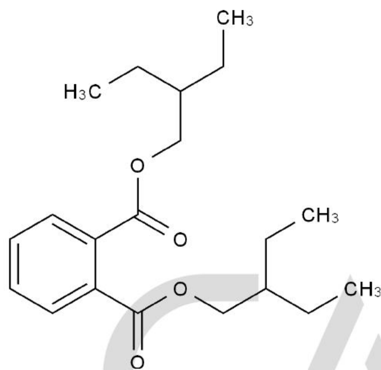
Chemical Structure:
