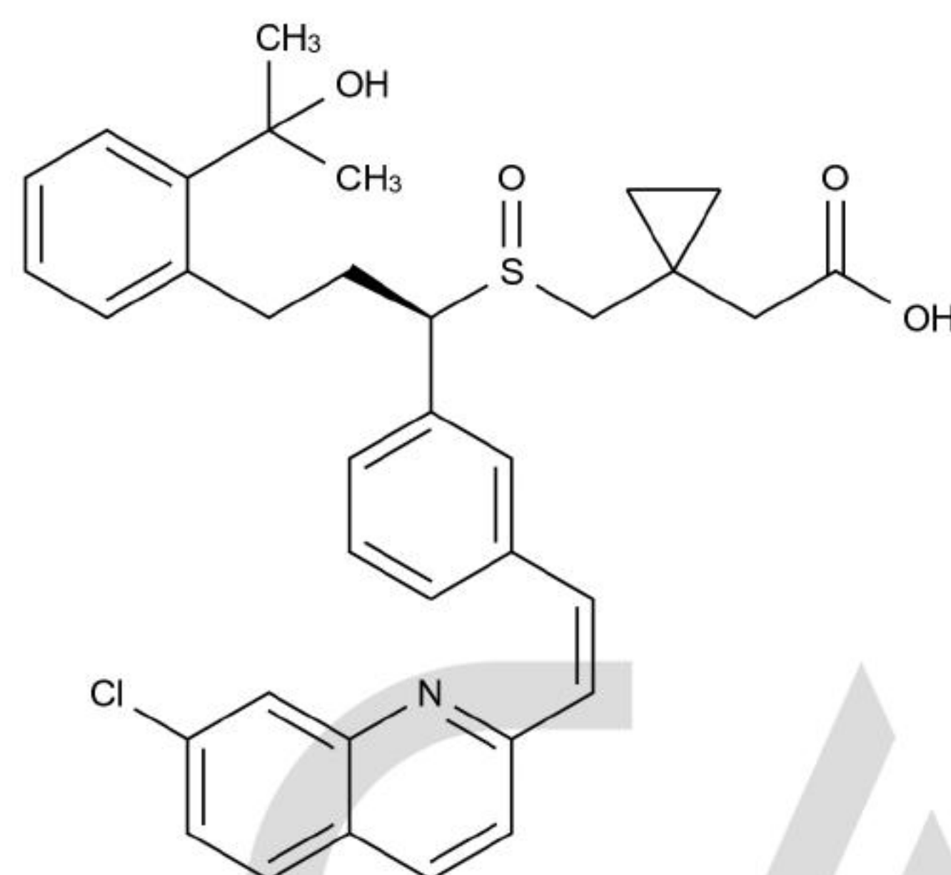
Chemical Structure:
