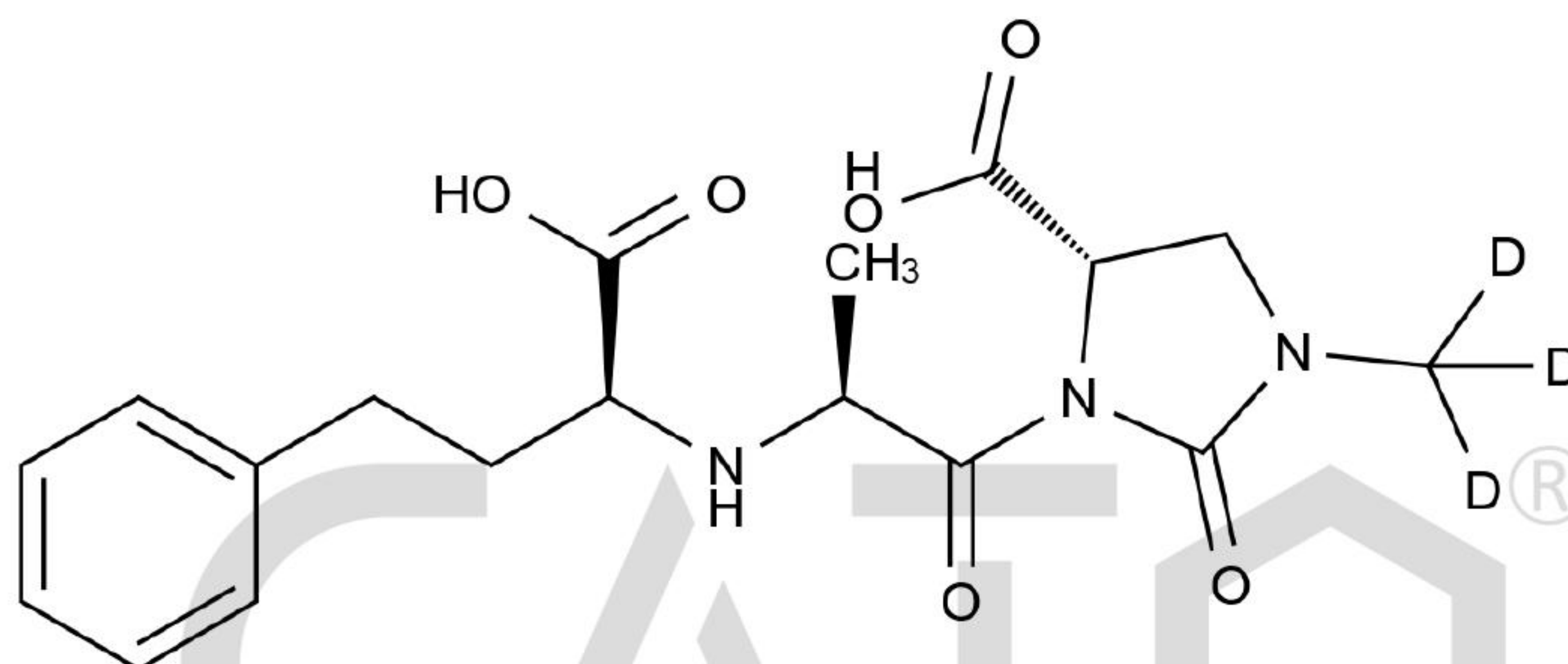
Chemical Structure:
