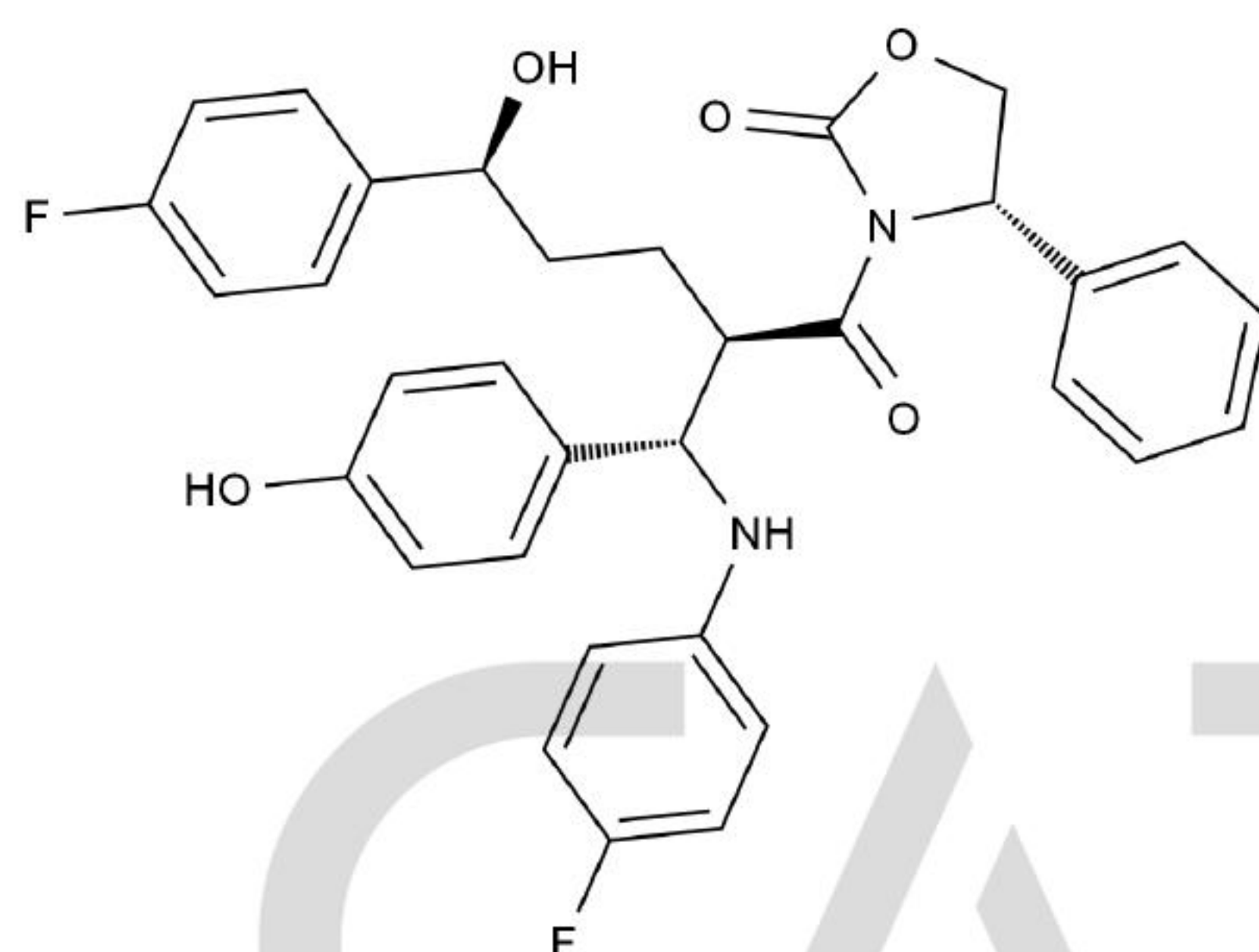
Chemical Structure:
