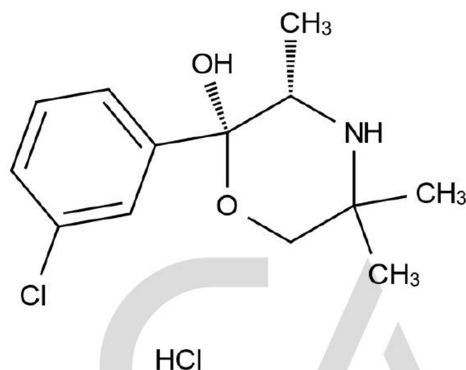
Chemical Structure:
