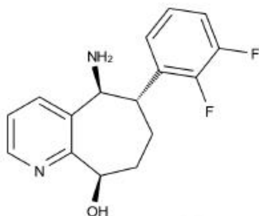
Chemical Structure:
