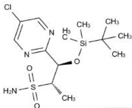
Chemical Structure:
