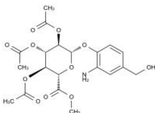
Chemical Structure:
