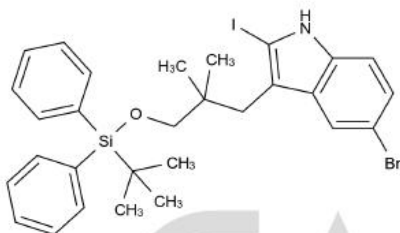
Chemical Structure:
