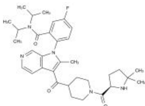
Chemical Structure:
