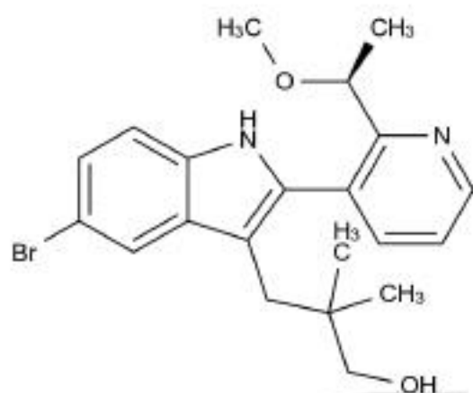
Chemical Structure:
