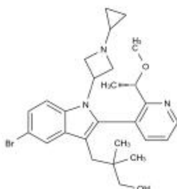
Chemical Structure:
