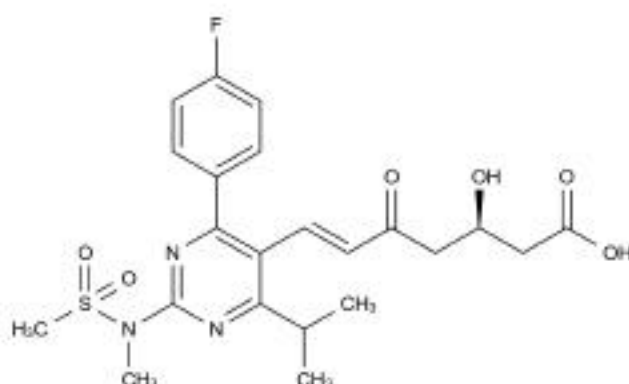
Chemical Structure:
