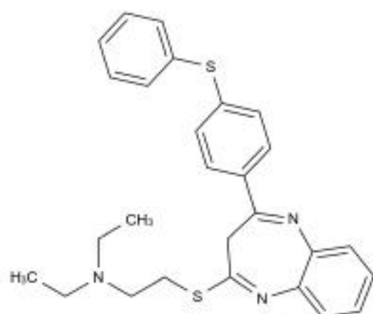
Chemical Structure:
