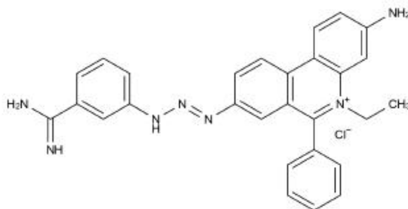
Chemical Structure:
