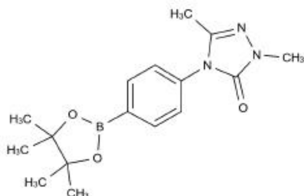
Chemical Structure:
