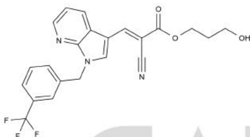
Chemical Structure:
