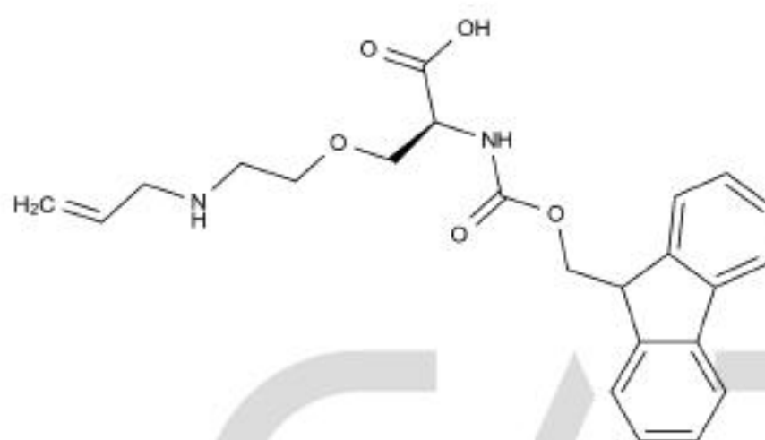
Chemical Structure:
