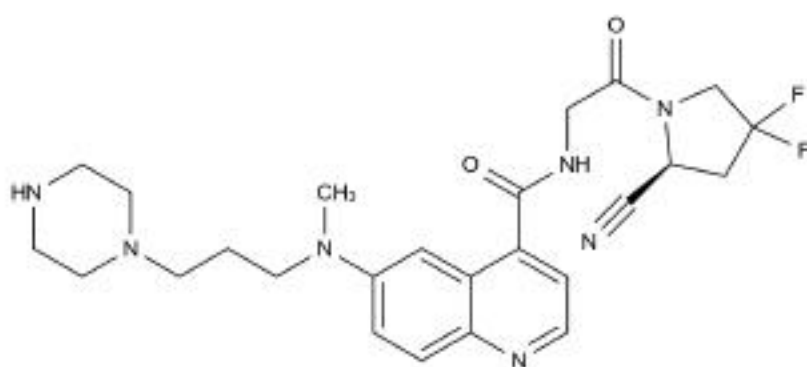
Chemical Structure:
