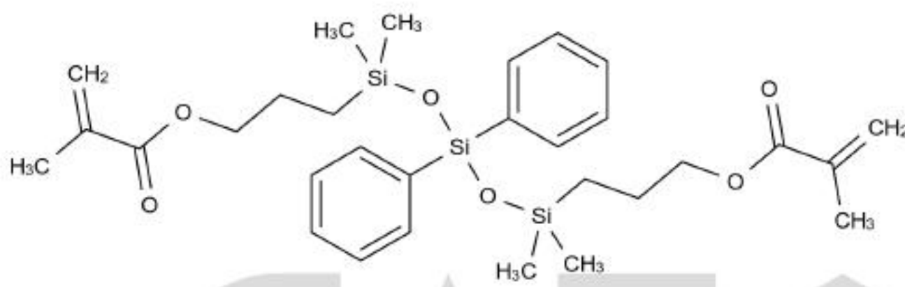
Chemical Structure:
