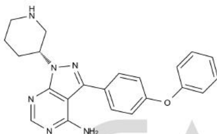
Chemical Structure:
