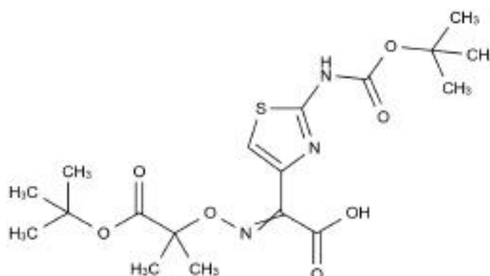
Chemical Structure:
