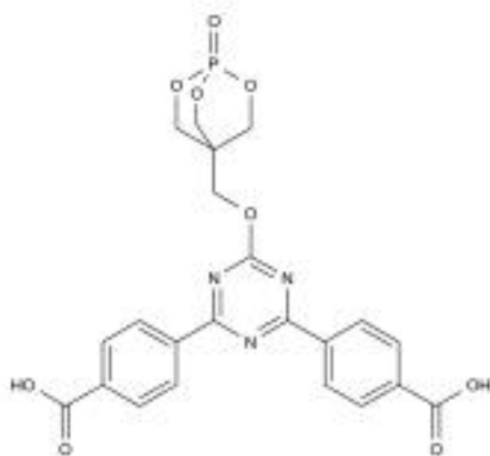
Chemical Structure:
