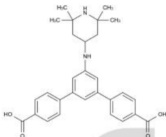
Chemical Structure:
