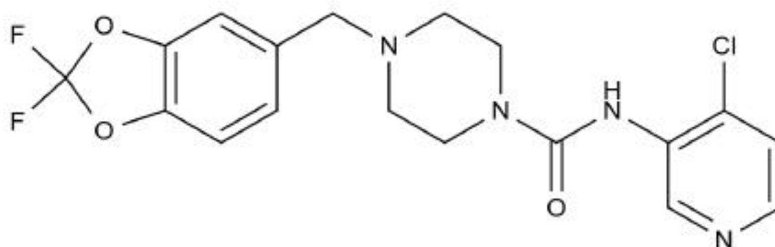
Chemical Structure:
