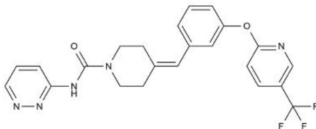
Chemical Structure:
