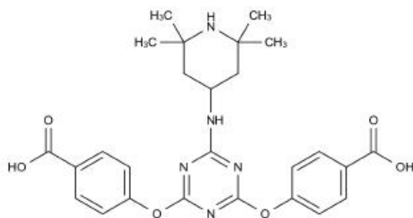
Chemical Structure:
