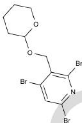
Chemical Structure:
