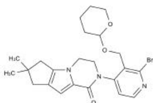
Chemical Structure:
