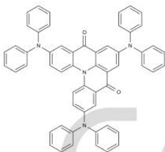
Chemical Structure:
