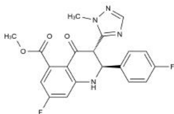
Chemical Structure:
