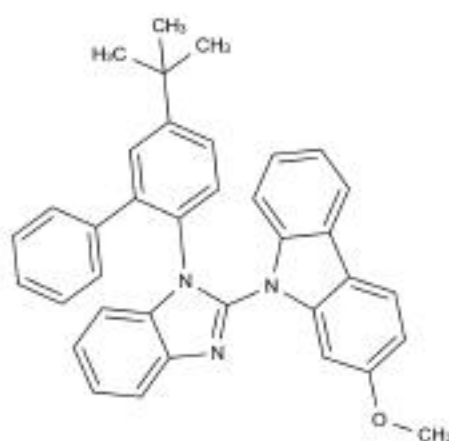
Chemical Structure:
