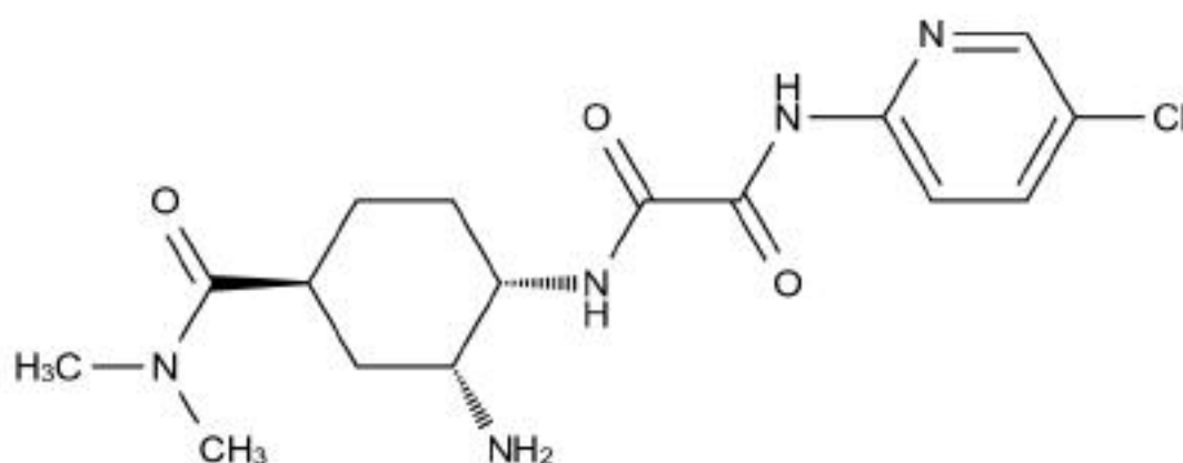
Chemical Structure:
