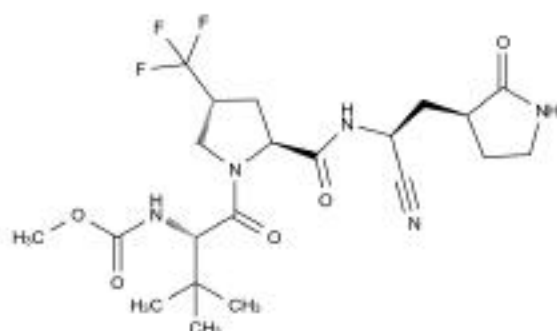
Chemical Structure:
