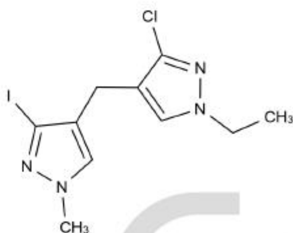
Chemical Structure:
