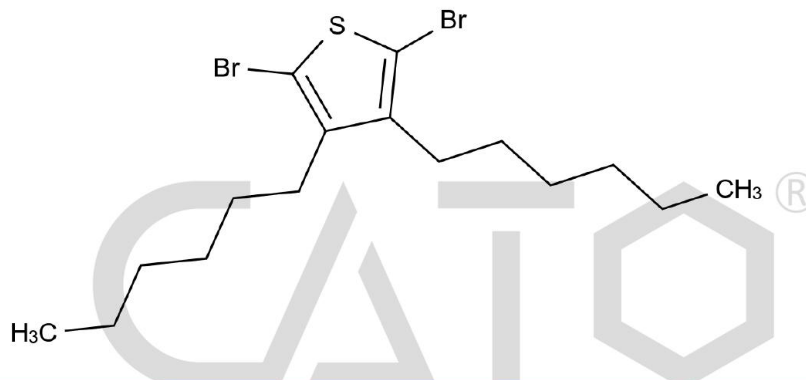
Chemical Structure:
