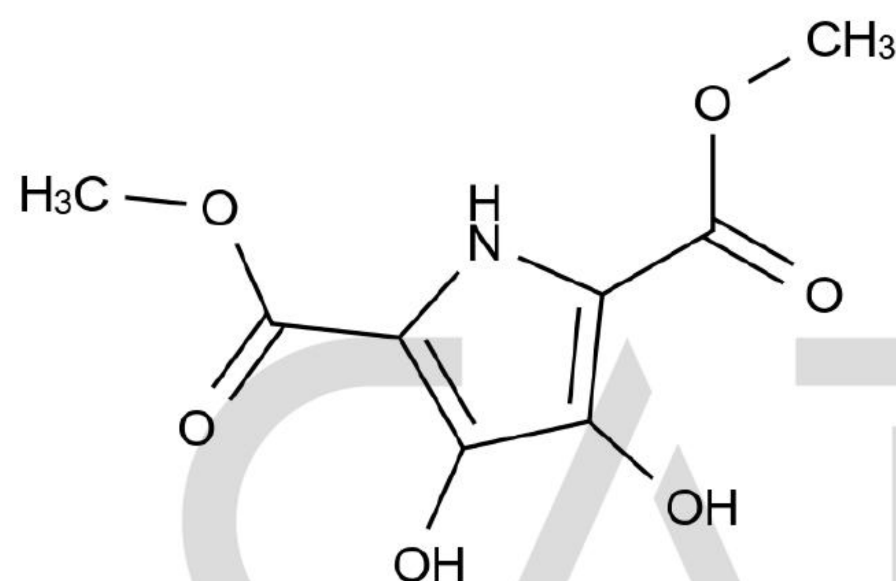
Chemical Structure:
