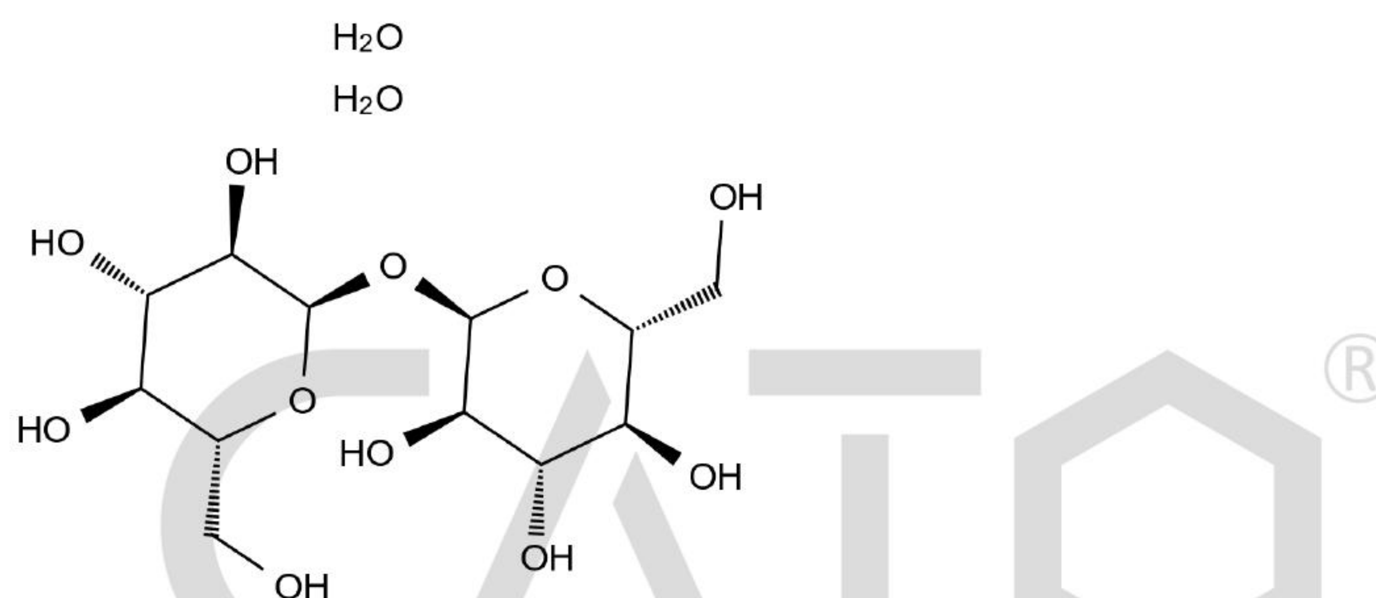
Chemical Structure:
