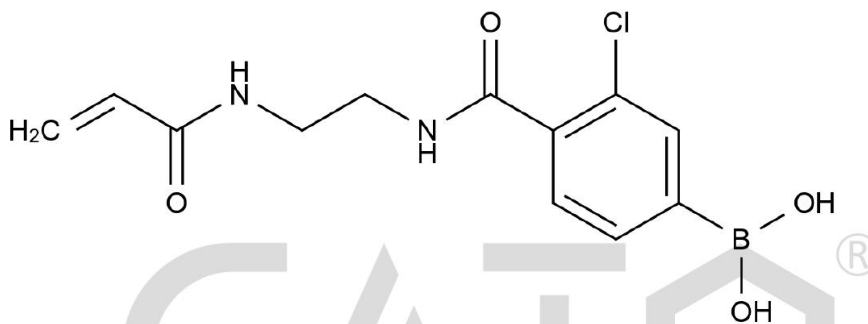
Chemical Structure:
