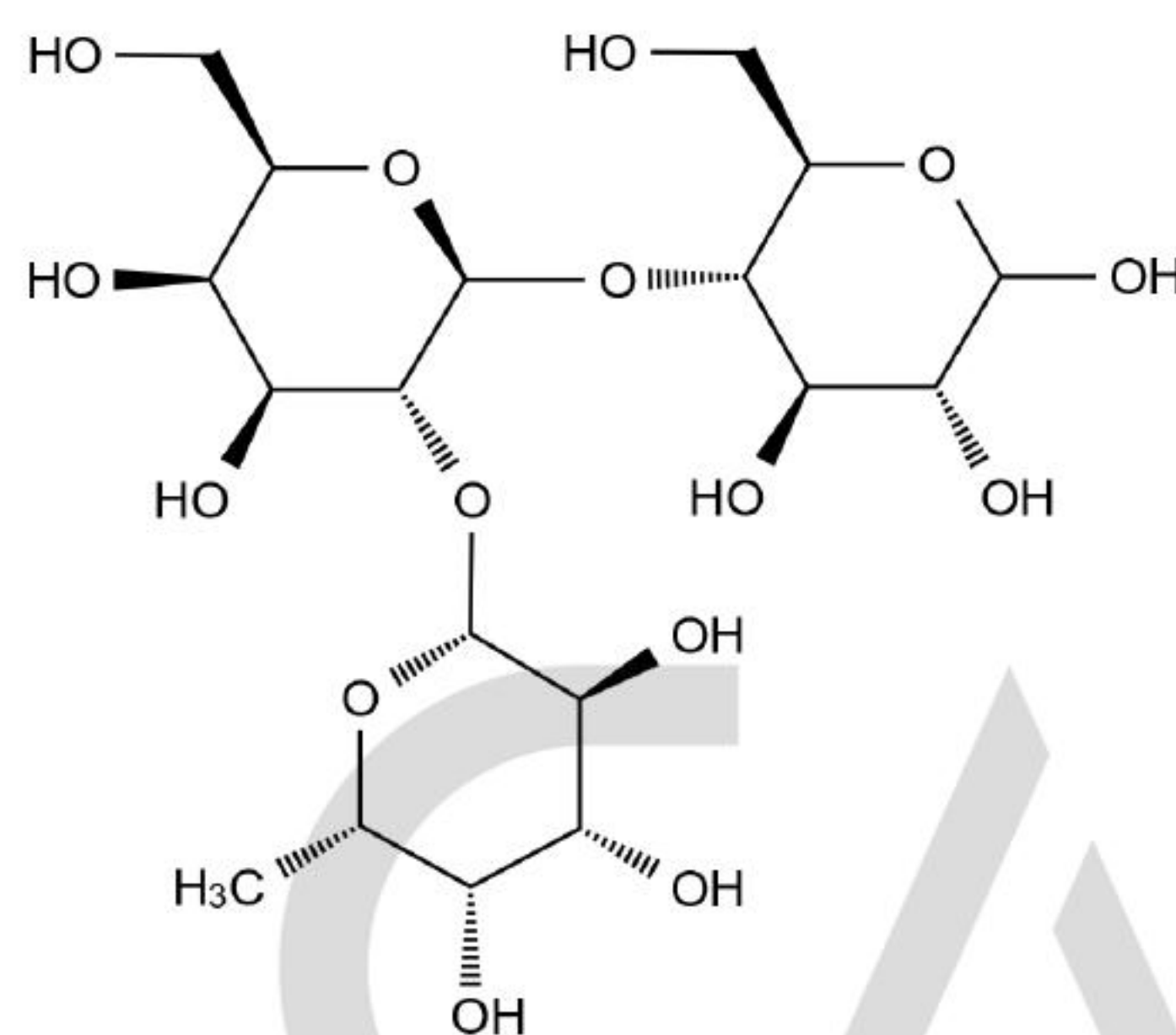
Chemical Structure:
